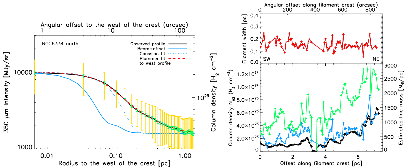
Fig. 2. (a) Median radial intensity profile of the NGC 6334 filament (black solid curve) measured perpendicular to, and on the western side of, the filament crest shown as a magenta curve in Fig. 1. The yellow error bars visualize the (\pm 1\sigma) dispersion of the distribution of radial intensity profiles observed along the filament crest, while the smaller green error bars represent the standard deviation of the mean intensity profile (the data points and error bars are spaced by half a beam width). The blue solid curve shows the effective beam profile of the ArTéMiS 350 \mu\text{m} data as measured on Mars, on top of a constant level corresponding to the typical background intensity level observed at large radii. The blue dotted curve shows the best-fit Gaussian (+ constant offset) model to the inner part of the observed profile. The red dashed curve shows the best-fit Plummer model convolved with the beam as described in the text. (b) Upper panel : Deconvolved Gaussian FWHM width of the NGC 6334 filament as a function of position along the filament crest (from south-west to north-east), with one width measurement per independent ArTéMiS beam of 8'' (red crosses). Lower panel : Observed column density (black curve and left y-axis), background-subtracted mass per unit length (blue curve and right y-axis) derived from a Gaussian fit (cf. blue dotted curve in (a)) to the filament transverse profile, and background-subtracted mass per unit length (green curve and right y-axis) derived from integration of the observed transverse profile (cf. black curve in (a)) up to an outer radius of 0.7 pc (or \sim 80'' ) where the background starts to dominate, all plotted as a function of position along the filament crest.
