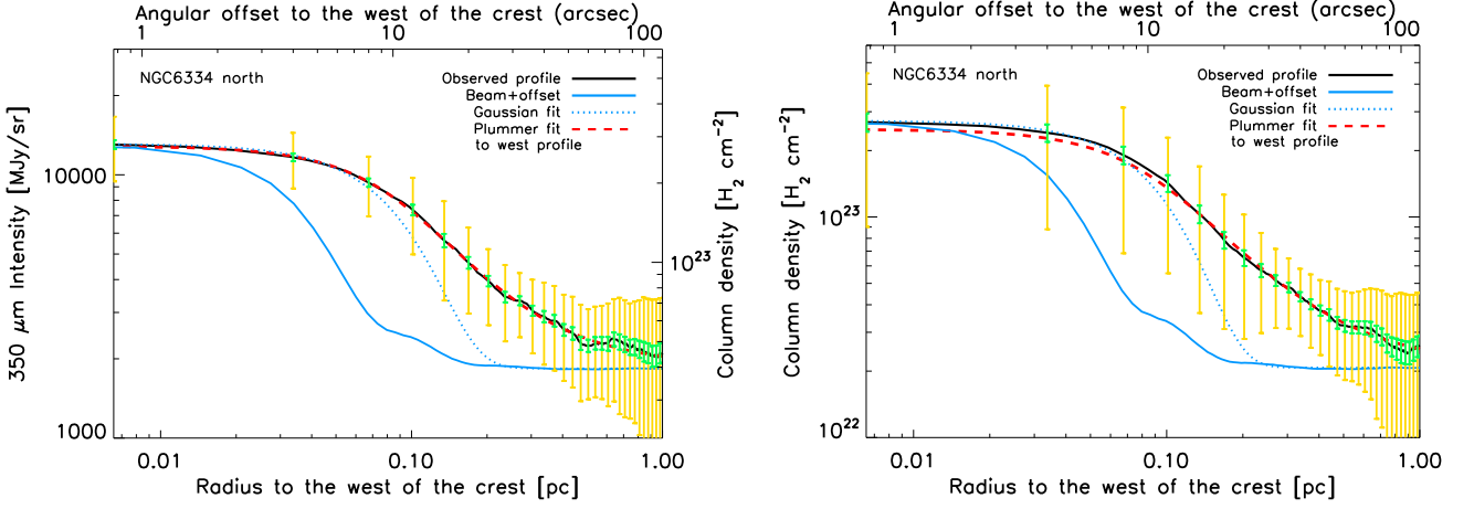
Fig. A.2. (a) Median radial intensity profile of the northern part of the NGC 6334 filament (black solid curve) measured in the combined ArTéMiS + SPIRE 350\ \mu\text{m} image (Fig. 1b) perpendicular to, and on the western side of, the filament crest shown as a cyan curve in Fig. A.1a. The yellow and green error bars are as in Fig. 2. The blue solid curve shows the effective beam profile of the ArTéMiS 350\ \mu\text{m} data as measured on Mars, on top of a constant level corresponding to the typical background intensity level observed at large radii. The blue dotted curve shows the best-fit Gaussian (+ constant offset) model to the inner part of the observed profile. The red dashed curve shows the best-fit Plummer model convolved with the beam [cf. Sect. 3 and Eq. (1)]. (b) Same as in (a) but for the median radial column density profile of the northern part of the filament derived from the approximate column density map shown in Fig. A.1a.
