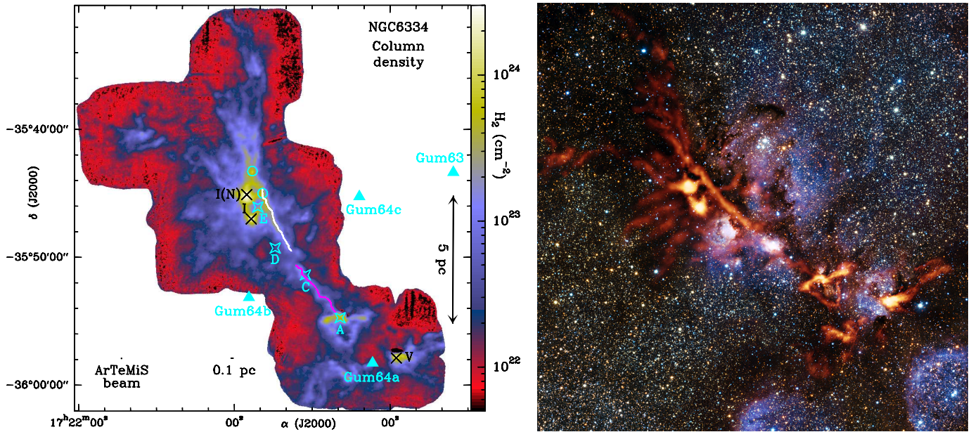
Fig. A.1. (a) Approximate \text{H}_2 column density map of the central part of the NGC 6334 star-forming complex derived from the combined ArTéMiS + SPIRE 350 \mu\text{m} image shown in Fig. 1b, assuming optically thin dust emission at the temperature given by the Herschel /HOBYS dust temperature map of Tigé et al. (2016) (see also Russeil et al. 2013). The effective angular resolution is 8'' (HPBW). The crest of the northern part of the NGC 6334 main filament as traced by the DisPerSE algorithm (Sousbie 2011) is marked by the white curve, while the crest of the southern part is shown by the magenta curve. Black crosses and roman numerals (I, V) denote bright far-infrared sources (Kraemer & Jackson 1999). Cyan open circles mark two candidate starless “massive dense cores” from Tigé et al. (2016). Cyan open diamonds and alphabetical letters A–E indicate compact HII regions detected in the 6 cm radio continuum with the VLA (Rodríguez et al. 1982), and cyan filled triangles mark diffuse HII regions traced as diffuse \text{H}\alpha emission nebulosities (Gum 1955). (b) ArTéMiS 350 \mu\text{m} image (orange) overlaid on a view of the same region taken at near-infrared wavelengths with the ESO VISTA telescope (see ESO photo release http://www.eso.org/public/images/eso1341a/ – Credit: ArTéMiS team/ESO/J. Emerson/VISTA).
